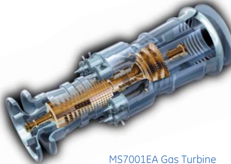
MS7001EA Gas Turbine
